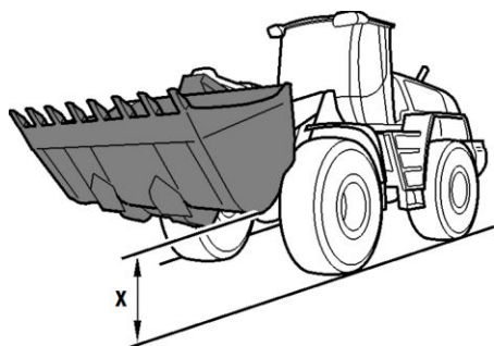
Position de transport
